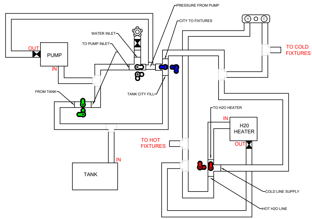
LOOKING AT THE FRONT OF THE PANEL
