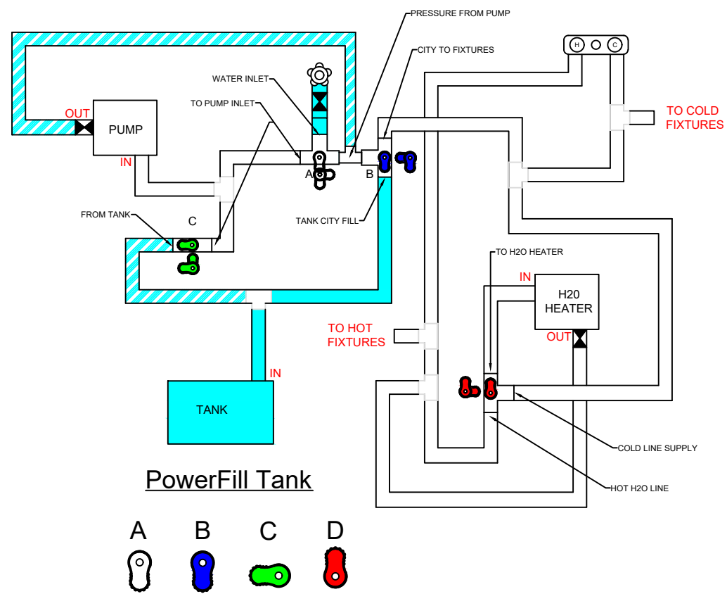
LOOKING AT THE FRONT OF THE PANEL
