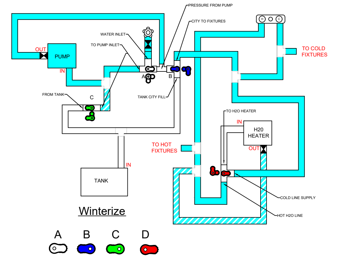
LOOKING AT THE FRONT OF THE PANEL
